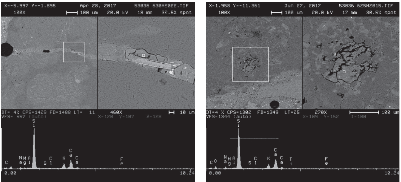
Figure 7 Backscattered electron (BSE) images with EDS spectra of ASR gel within pockets in Coarse Aggregate 2
