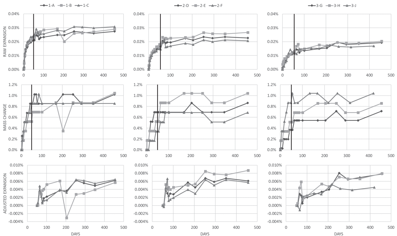
Figure 9 Raw expansion, mass change, and adjusted expansion for 150-mm diameter cores stored over water at 38 °C.
