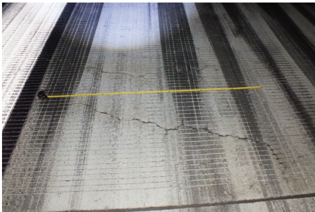
Figure 2 Example of surface cracking
