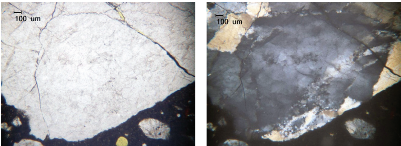
Figure 6 Polarized light micrographs in different light modes of reactive metagranite containing strained quartz found in Coarse Aggregate 1 and Intermediate Aggregate 1
