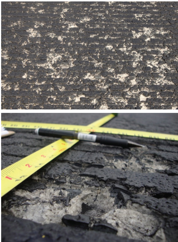
Figure 1 Examples surface distress (popouts and loss of paste)
