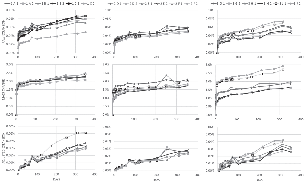
Figure 8 Raw expansion, mass change, and adjusted expansion for 50-mm diameter cores stored in 1N NaOH at 38 °C
