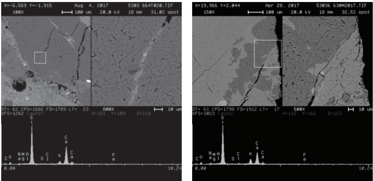
Figure 5 Backscattered electron (BSE) images with EDS spectra of ASR gel within cracks in Coarse Aggregate 1
